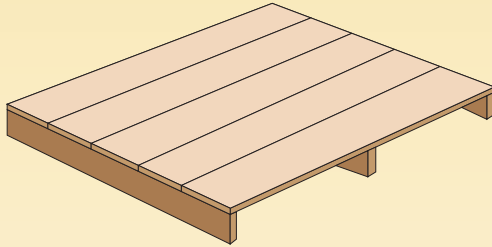
Four way entry pallet close boarded, 3 base
